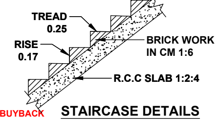
STAIRCASE DETAILS
