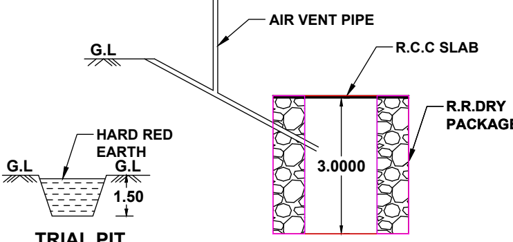
SECTION OF SOAKPIT
