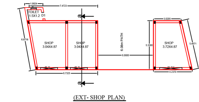
(EXT- SHOP PLAN)
