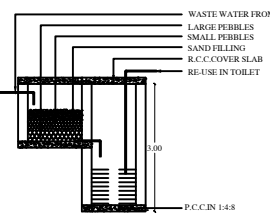
RECYCLING OF WASTE WATER FROM BATH
