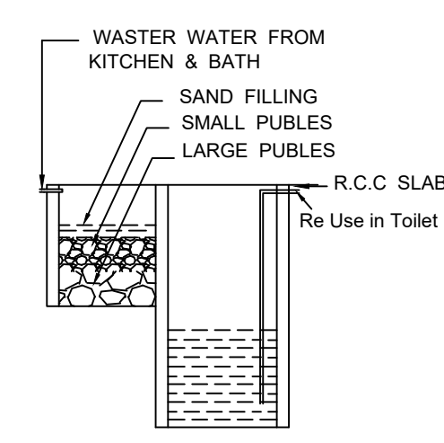
RECYCLING OF WASTE WATER KITCHEN & BATH ROOM
