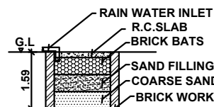
RAIN WATER HARVESTING PIT
