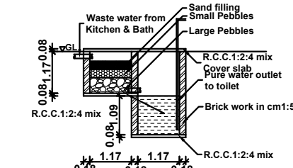
WASTE WATER RECYCLING SYSTEM
