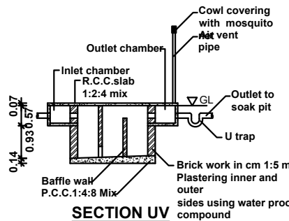
SECTION UV
