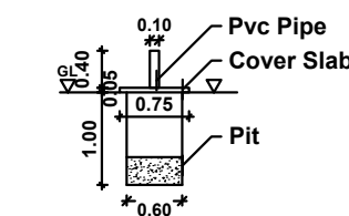
SOLID WASTE COMPOST PIT
