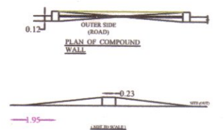
PLAN OF COMPOUND WALL
