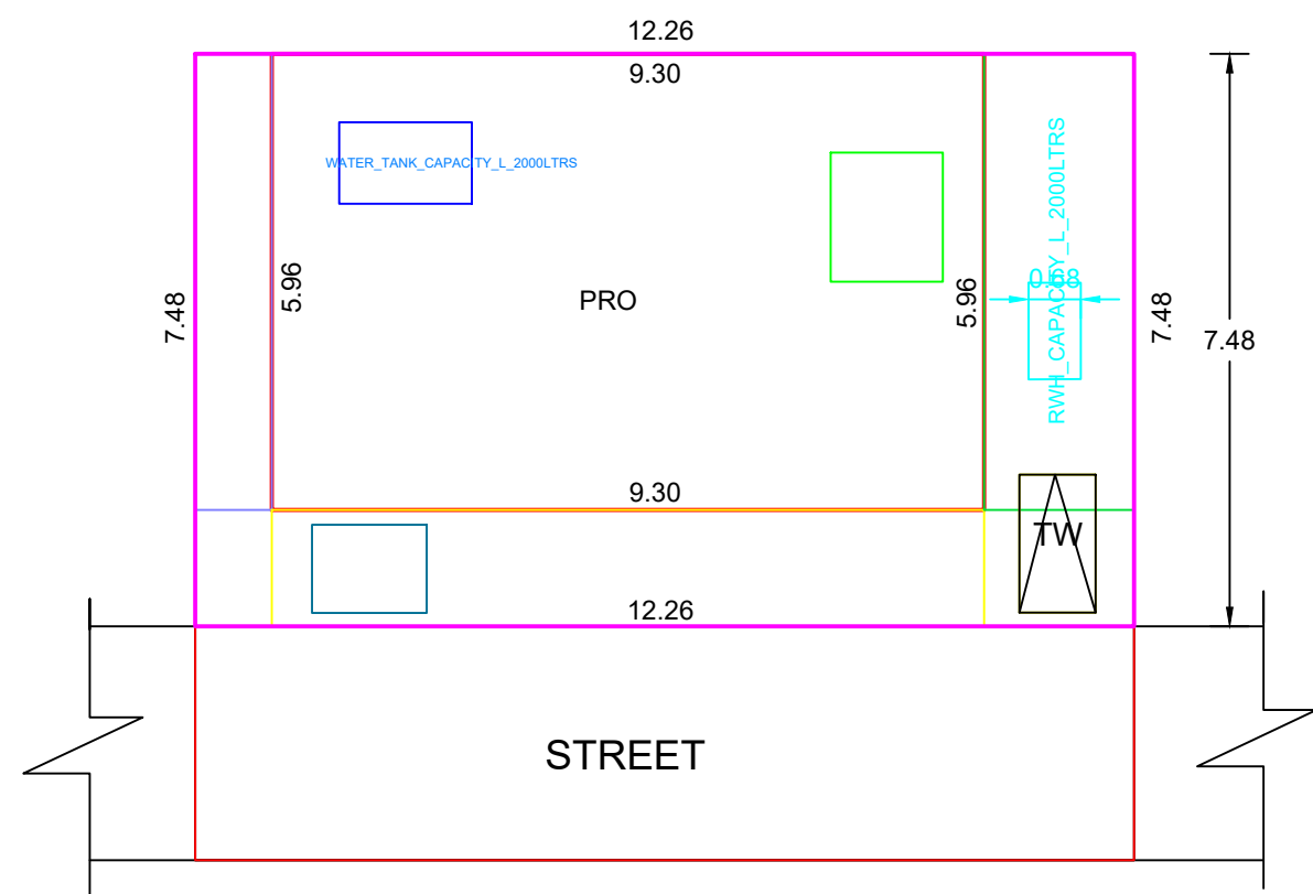
SITE PLAN
