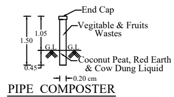
PIPE COMPOSTER
