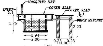
SECTION OF SEPTIC TANK
