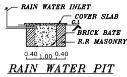
RAIN WATER PIT
