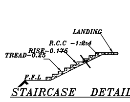
STAIRCASE DETAIL
