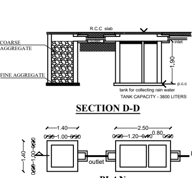
DETAILS OF THE RAIN WATER COLLECTING TANK
