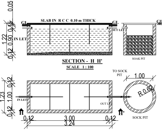
PLAN SEPTIC TANK & SOAK PIT
