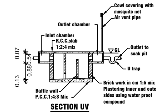
SECTION UV
