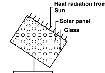
SOLAR SYSTEM
