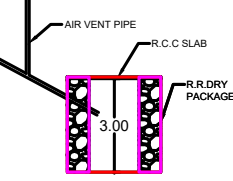
SECTION OF SOAKPIT
