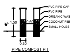
PIPE COMPOST PIT
