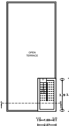
HEAD ROOM PLAN
