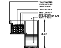
RECYCLING OF WASTE WATER FROM KITCHEN & BATHROOM
