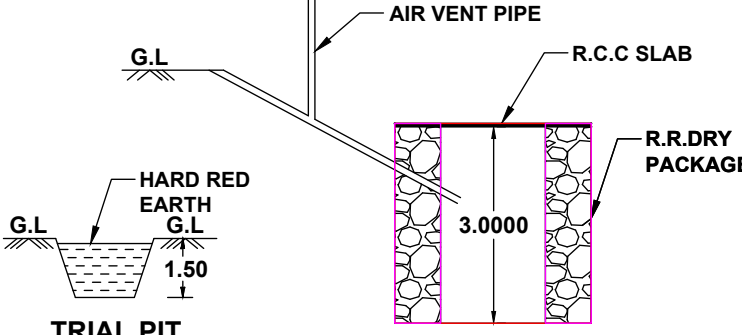
SECTION OF SOAKPIT
