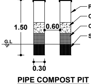
PIPE COMPOST PIT
