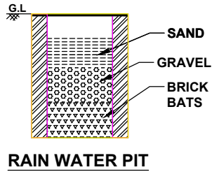
RAIN WATER PIT
