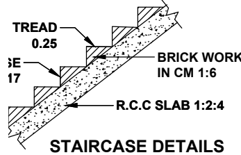
STAIRCASE DETAILS
