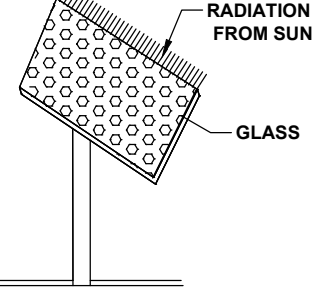
SOLAR DETAILS
