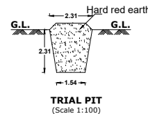
TRIAL PIT (Scale 1:100)
