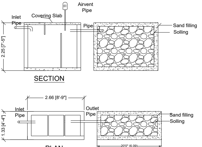
DETAILS OF SEPTIC TANK & DISPERSION TRENCH
