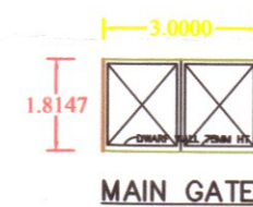
MAIN GATE
