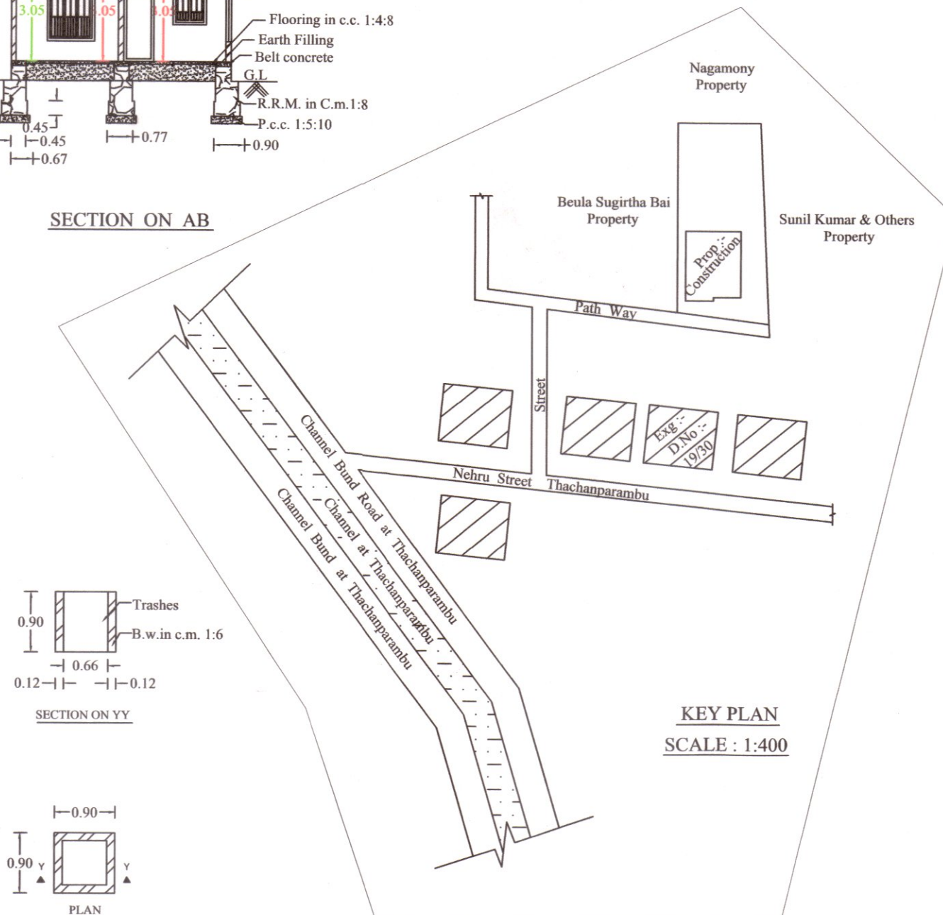
WASTE TRASH PIT
