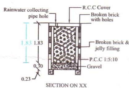
RAIN WATER HARVEST WELL
