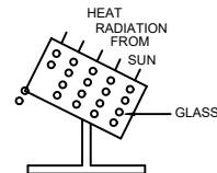
SOLAR SYSTEM
