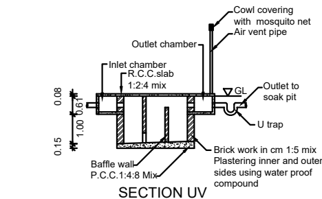
SECTION UV
