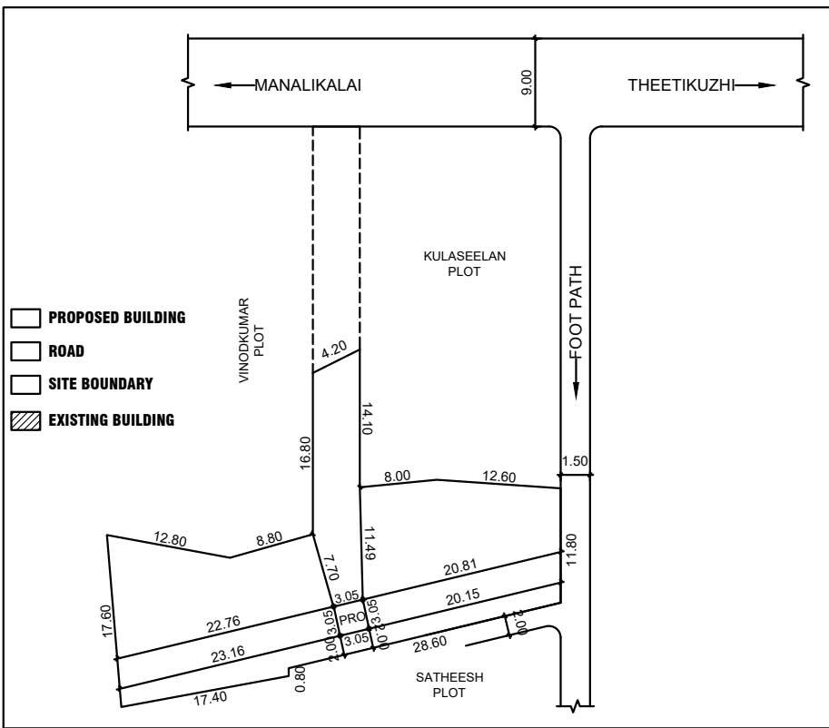
KEY PLAN SCALE:1:400
