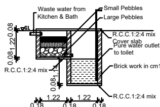
WASTE WATER RECYCLING SYSTEM
