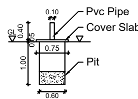
SOLID WASTE COMPOST PIT
