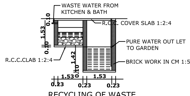
RECYCLING OF WASTE WATER SYSTEM
