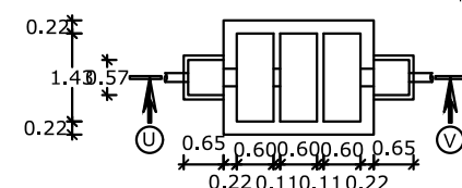
SECTION UV
