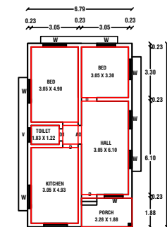
GROUND FLOOR PLAN SCALE 1:100 ALL DIMS ARE IN METER
