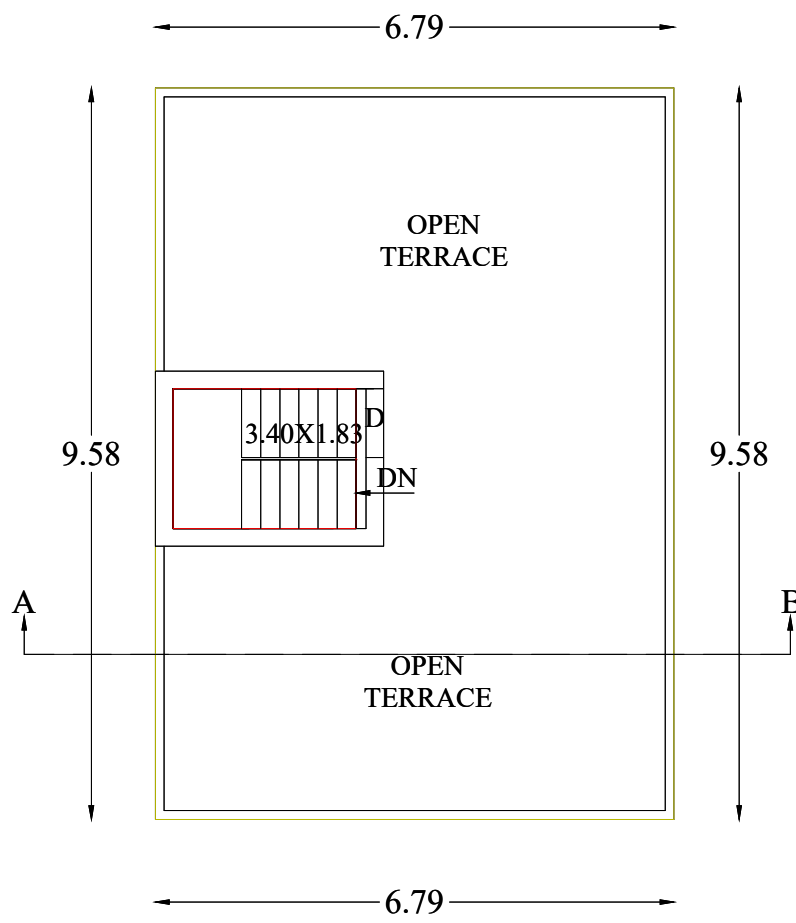
HEAD ROOM PLAN
