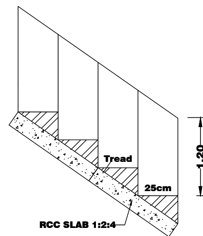
STAIR DETAILS
