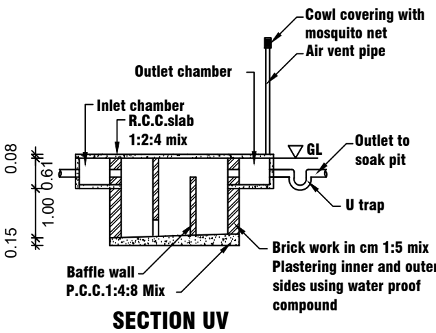
SECTION UV
