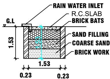
RAIN WATER HARVESTING PIT RWHP_CAPACITY_L=5000LTRS
