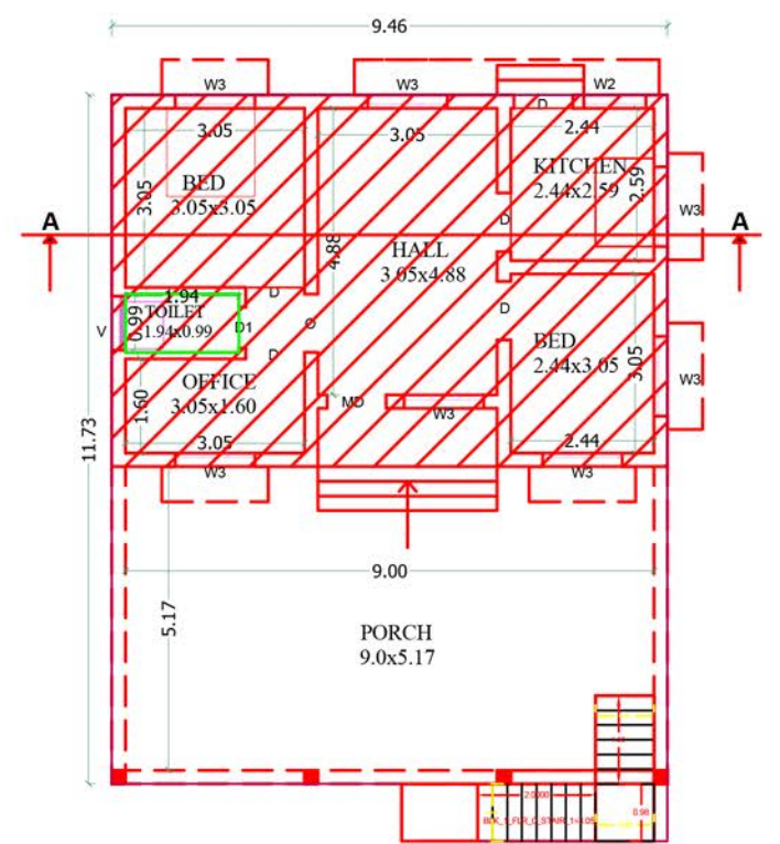
LOOR PLAN
