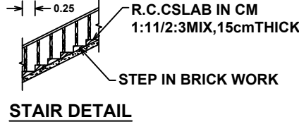
STAIR DETAIL
