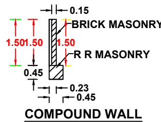
COMPOUND WALL
