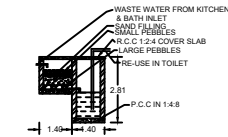
RECYCLING OF WASTE WATER KITCHEN & BATH ROOM
