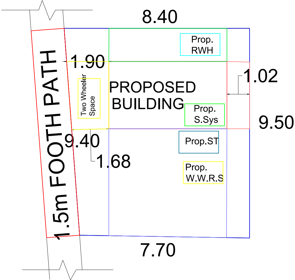
WASTE WATER RECYCLING SYSTEM
