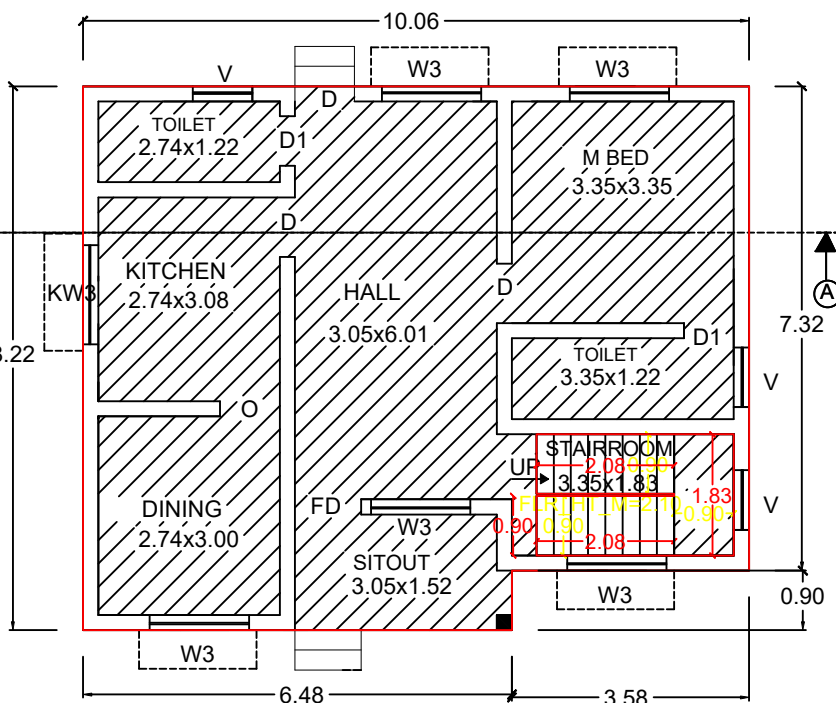
EX.GROUND FLOOR PLAN
