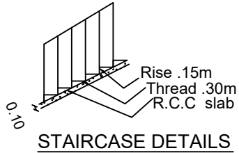
STAIRCASE DETAILS
