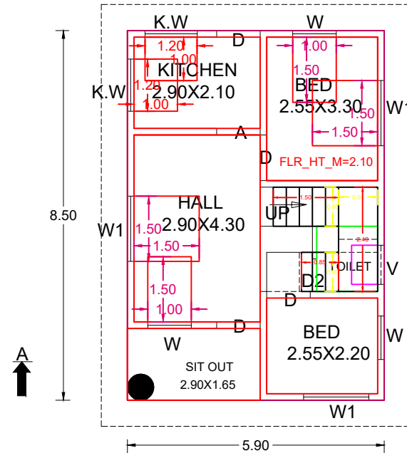
G.F. PLAN
