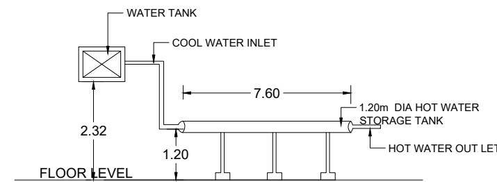
SOLAR WATER HEATING SYSTEM(S.W.H.S. DETAILS)
