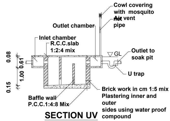
SECTION UV
