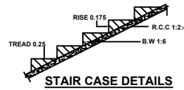
STAIR CASE DETAILS
