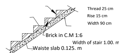
STAIR DETAILS
