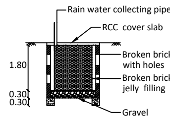
RAIN WATER HARVEST WELL SECTION
