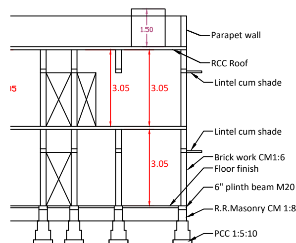
SECTION ON A-A [1:100]
