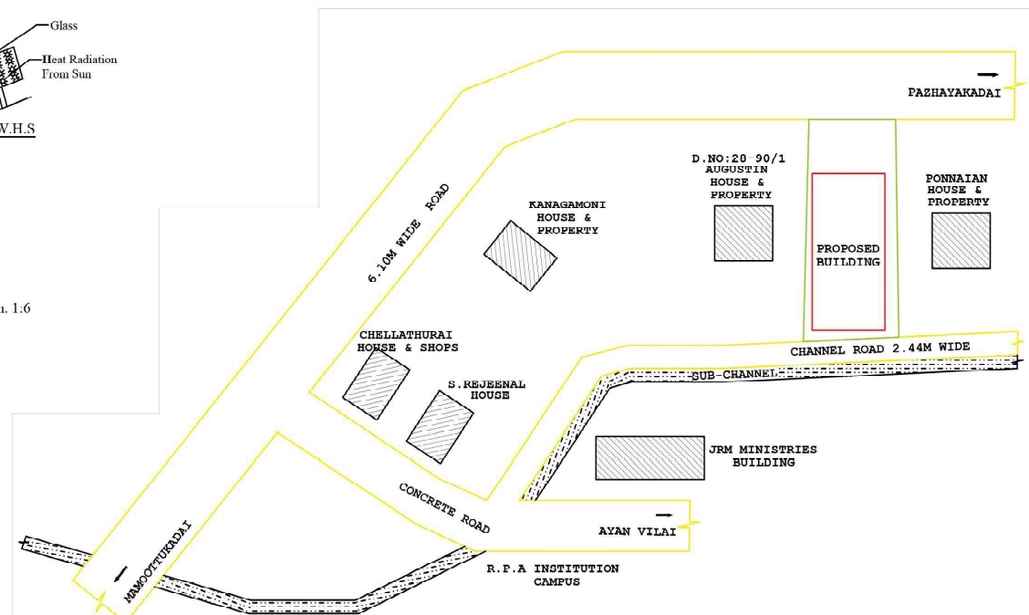
KEYPLAN (SCALE:1:300)
