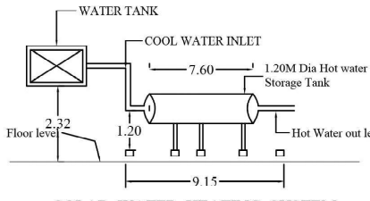
SOLAR WATER HEATING SYSTEM (S.W.H.S.DETAILS)
