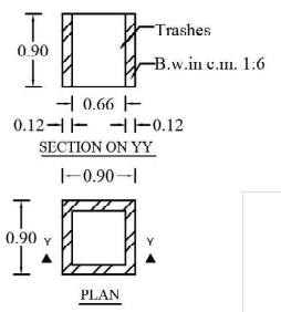
WASTE TRASH PIT
