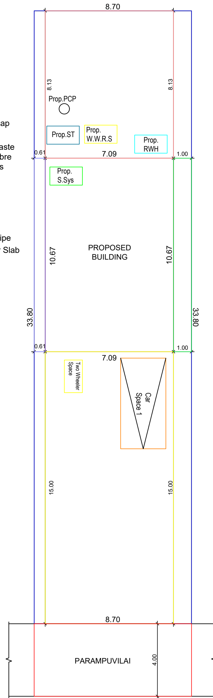
SITE PLAN
