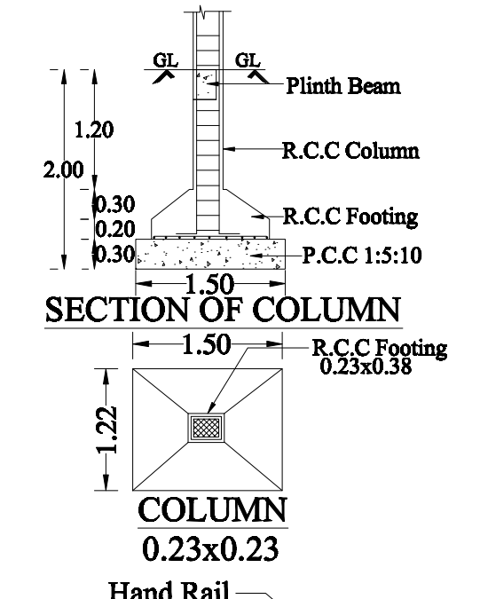
RAIN WATER PERCOLATION DRAWING TYPE -1A
