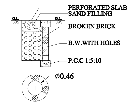
RAIN WATER PERCOLATION DRAWING TYPE -1A
