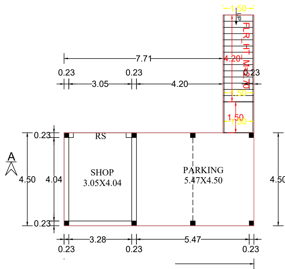
1ST FLOOR
