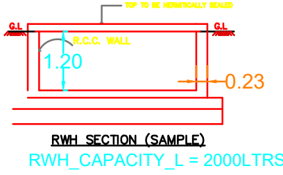
RWHL SECTION (SAMPLE) RWHL_CAPACITY_L = 2000LTRS
