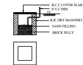
RAIN WATER HARVEST ARRANGEMENTS
