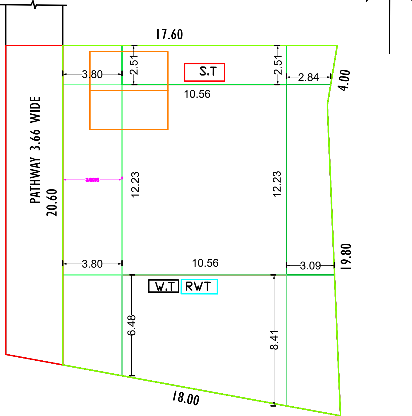
SITE PLAN
