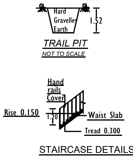
STAIRCASE DETAILS
