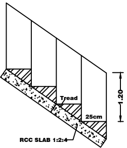
STAIR DETAILS
