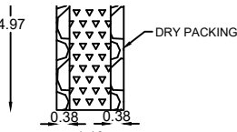
WASTE WATER TANK
