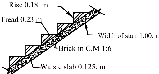
Stair Details
