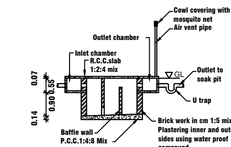
SECTION UV
