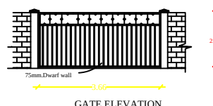
GATE ELEVATION
