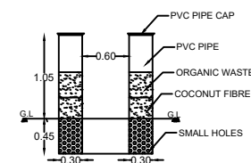
PIPE COMPOSIT PIT
