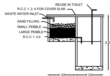
RECYCLING OF WASTE WATER
