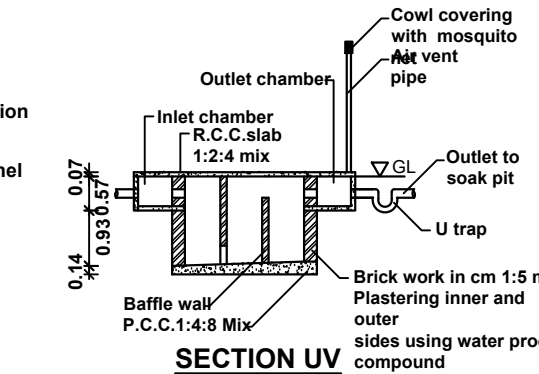
SECTION UV
