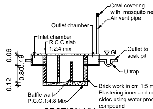
SECTION UV
