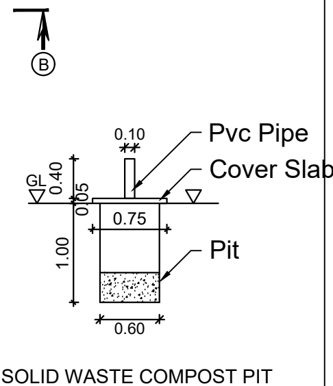
SOLID WASTE COMPOST PIT
