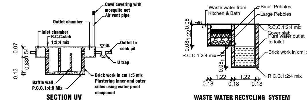
SECTION UV
