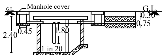
DETAILS OF SEPTIC TANK
