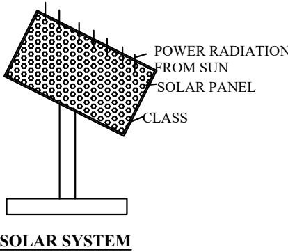
SOLAR SYSTEM
