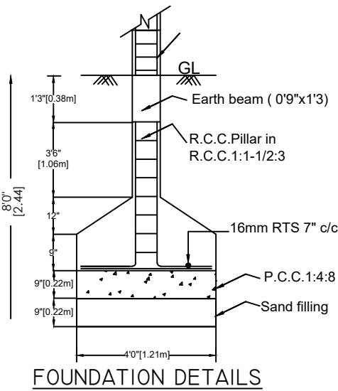
FOUNDATION DETAILS
